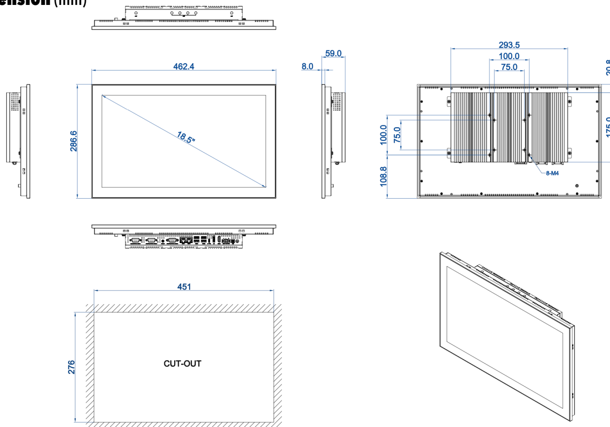
DIMENSIONAL DRAWING:TPC-DCT185D
