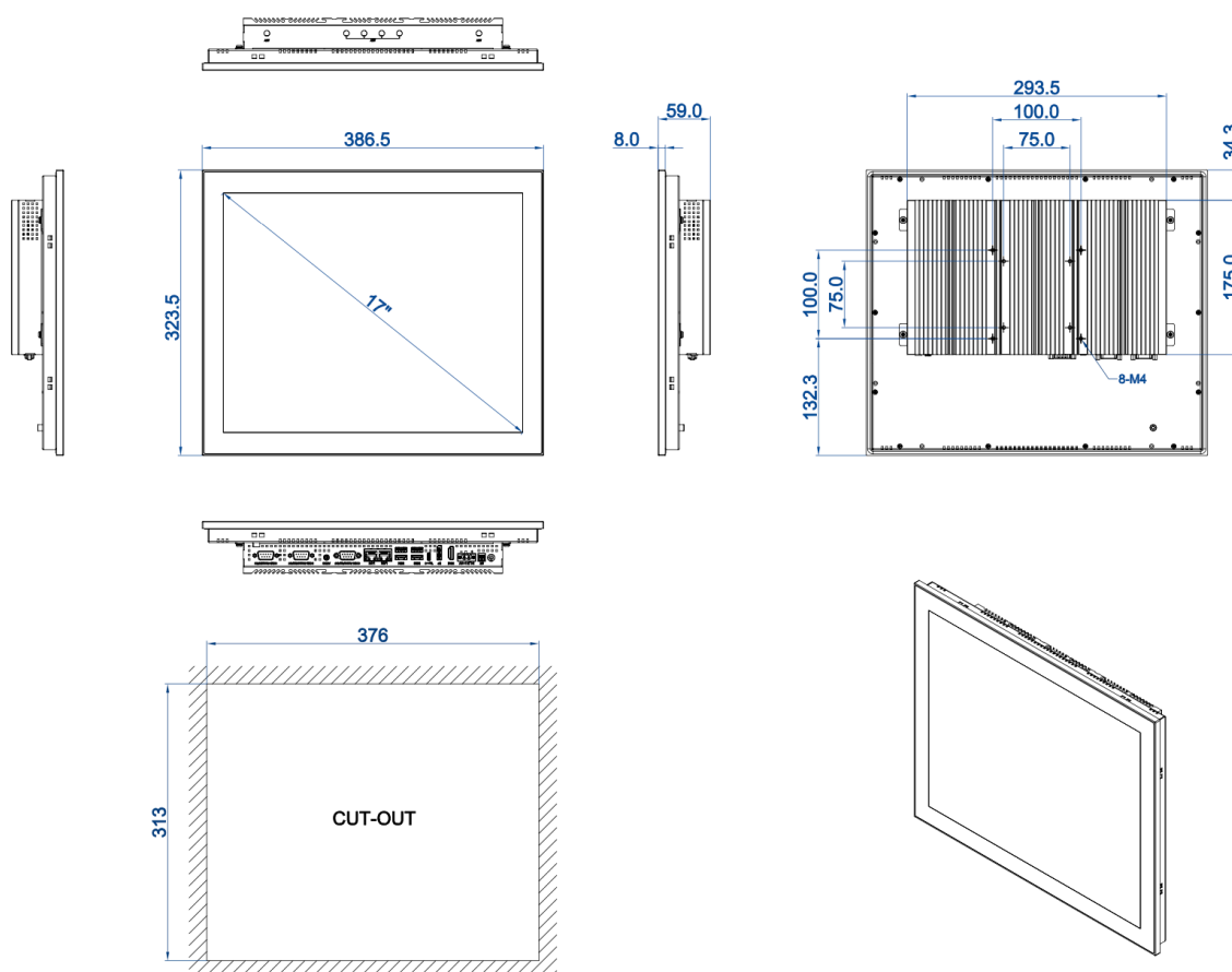
DIMENSIONAL DRAWING:TPC-DCT170D
