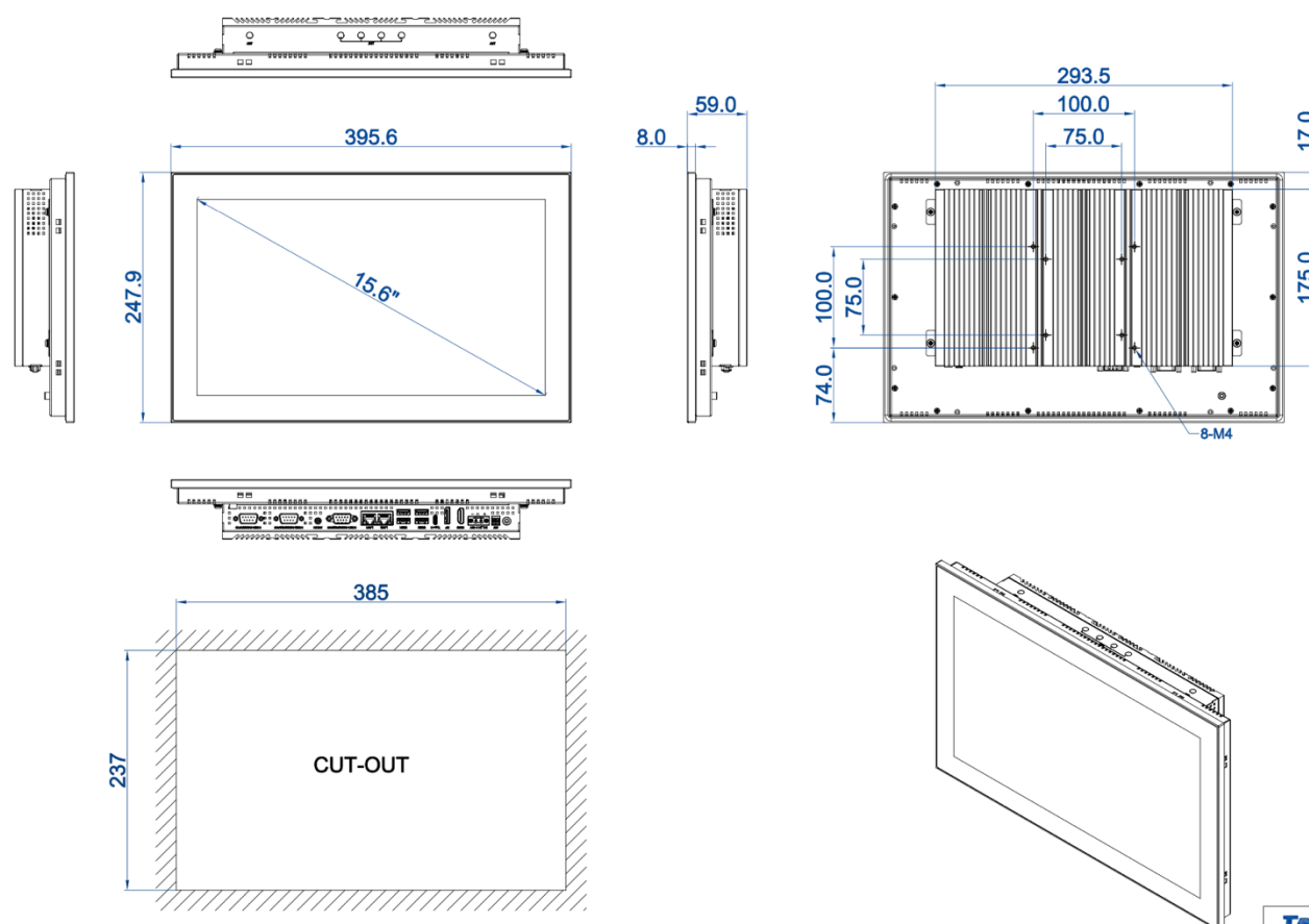
DIMENSIONAL DRAWING:TPC-DCT156D
