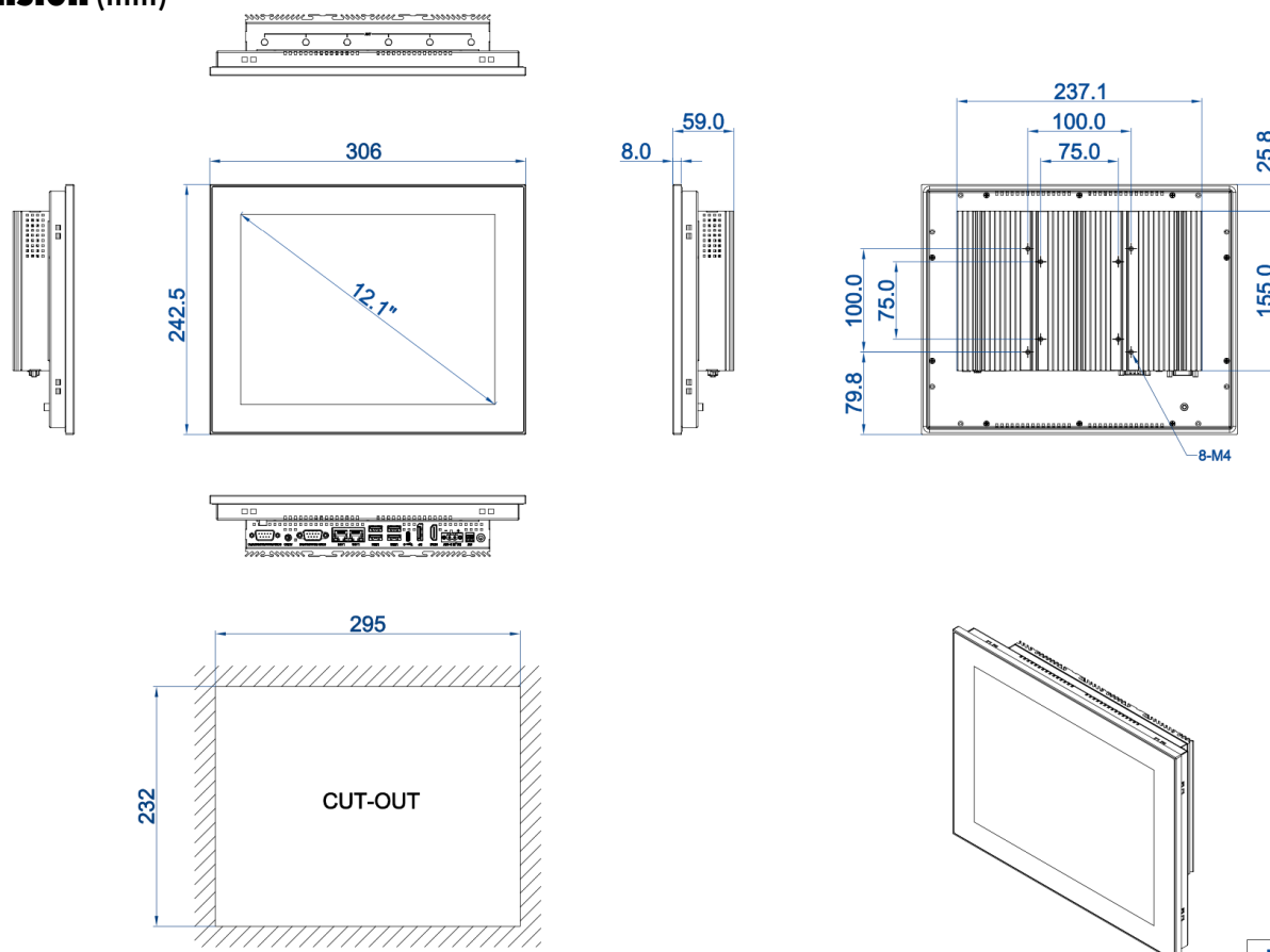
DIMENSIONAL DRAWING:TPC-DCT121D
